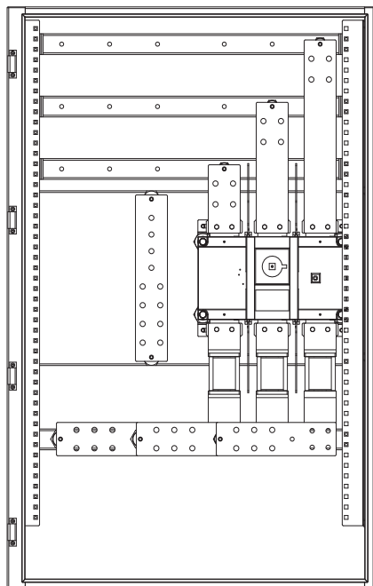
Internal View of AC Combiner Box
